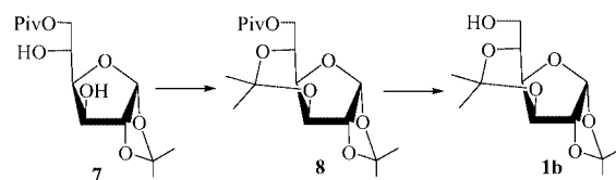
Scheme 2. Preparation of 1,2:3,5-di- O -isopropylidene-D-glucofuranose.
