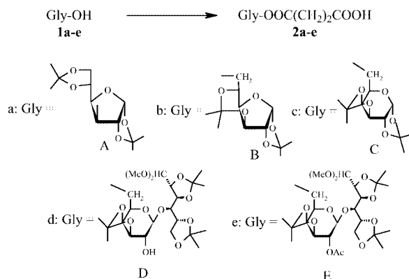
Scheme 1. Monosuccinates of protected glycidates.
