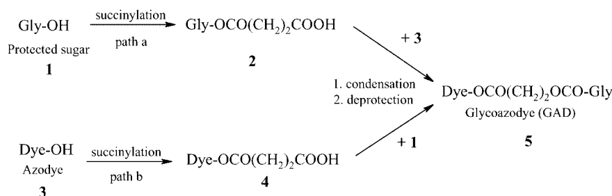
Figure 1. Schematic approaches to glycoazodyes (GADs).
