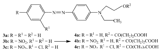
Scheme 3. Azodyes monosuccinates.
