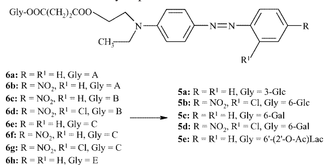
Scheme 4. Protected and deprotected GADs.
